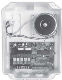
MV09 Control box
