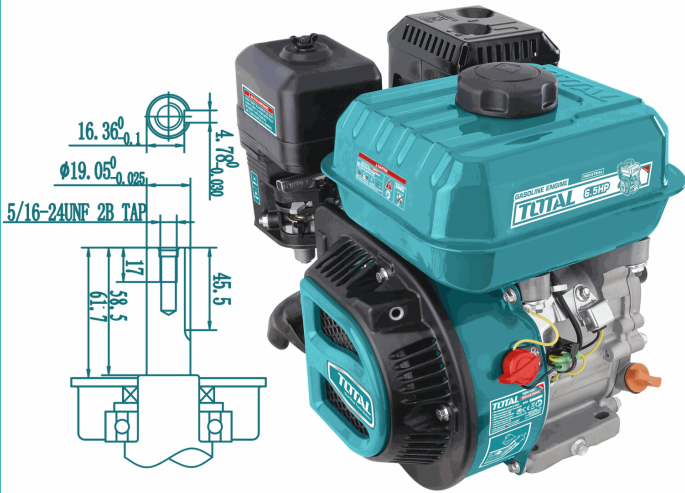
Low oil shutoff system
